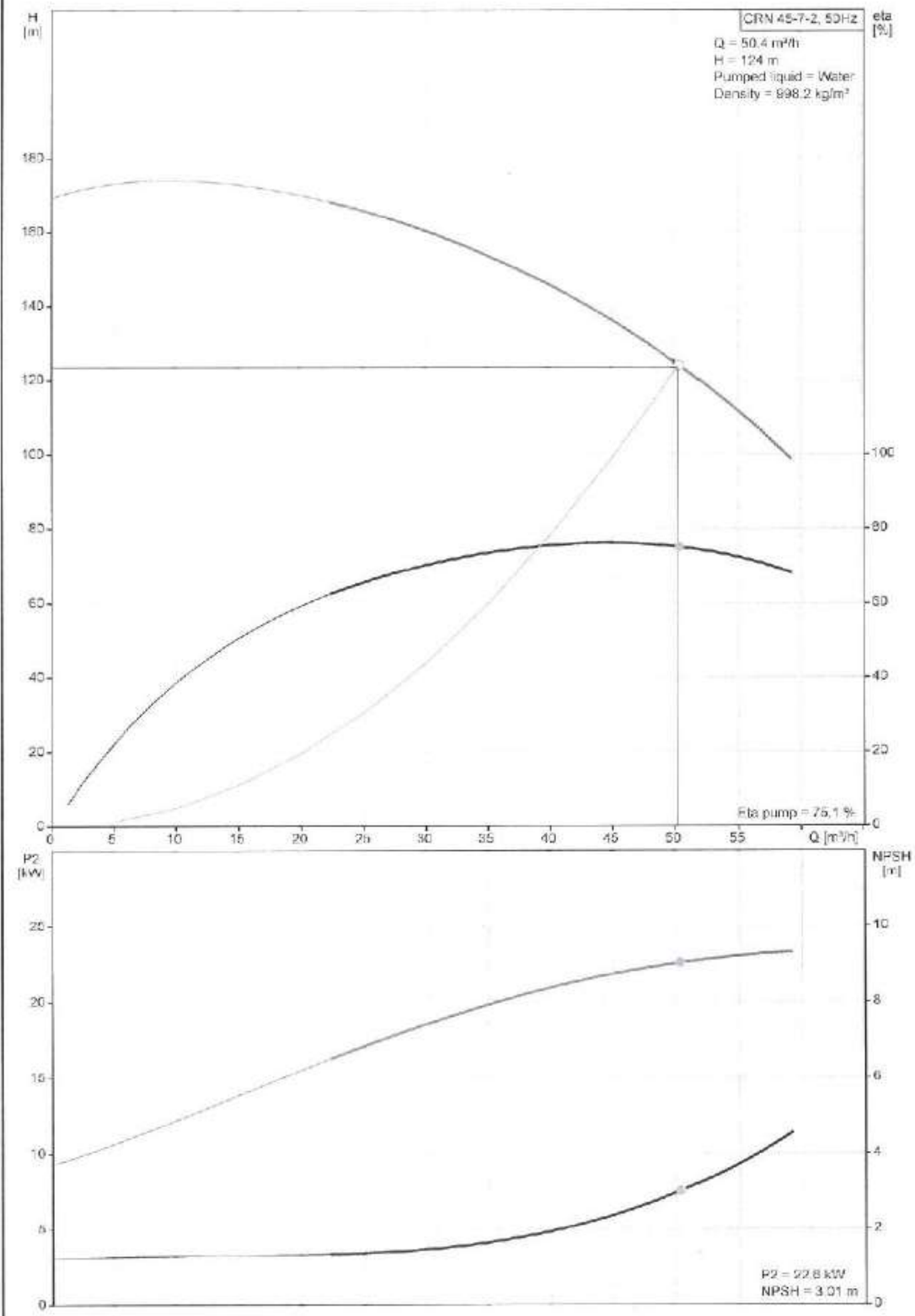
Performance curve of existing high pressure pump
